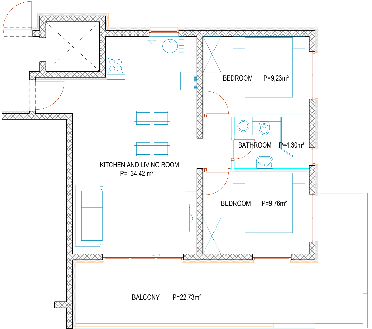
APARTMENT 3RD FLOOR P=77.08m 2
